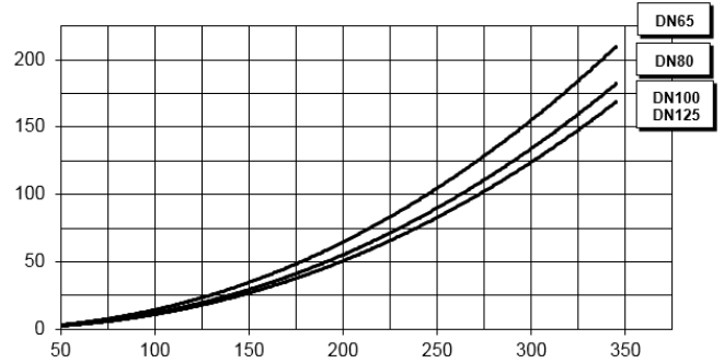
CAUDAL GAS METANO \text{Stm}^3/\text{h}
